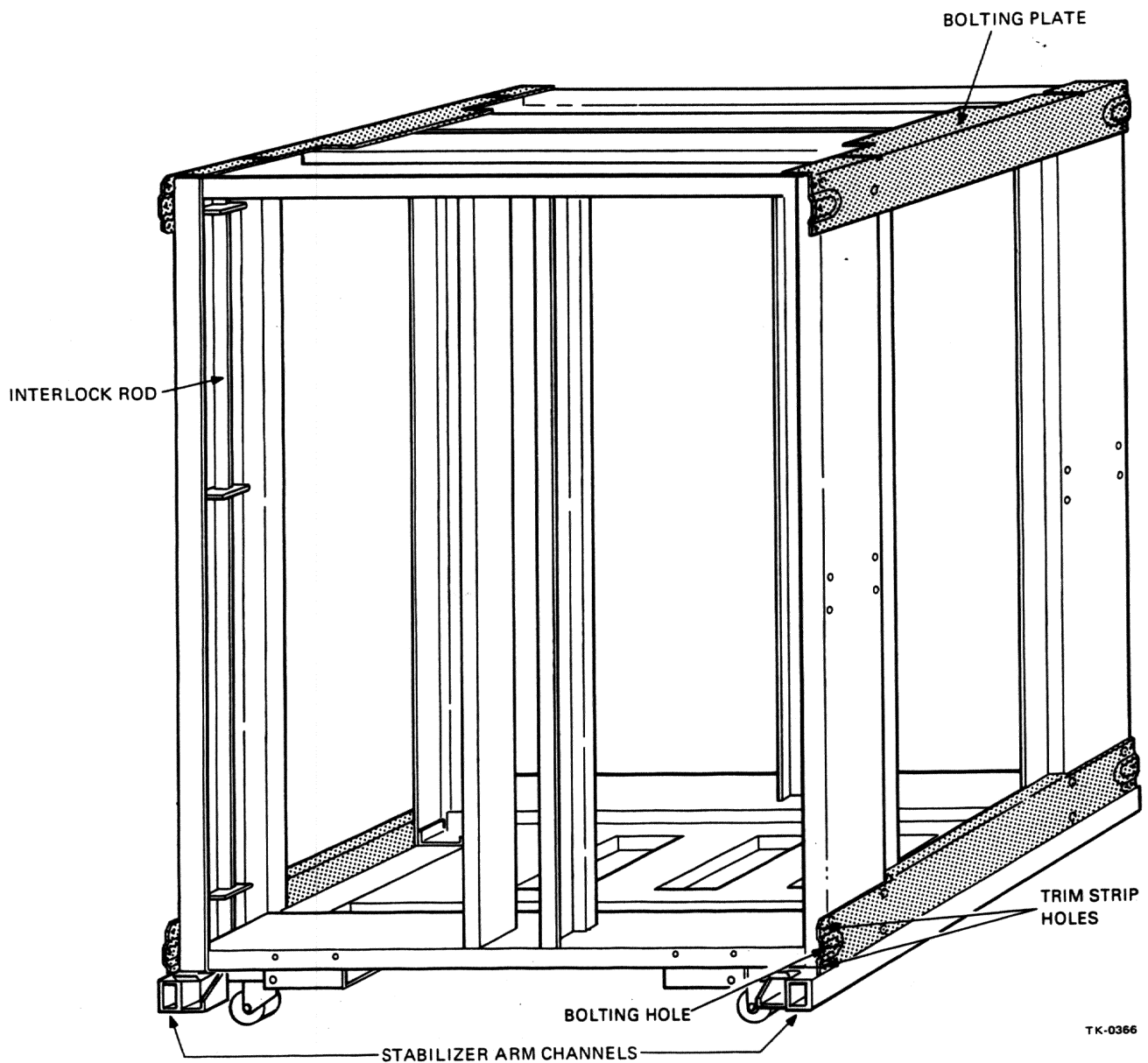
Figure 1-12 Cabinet Framework Details
