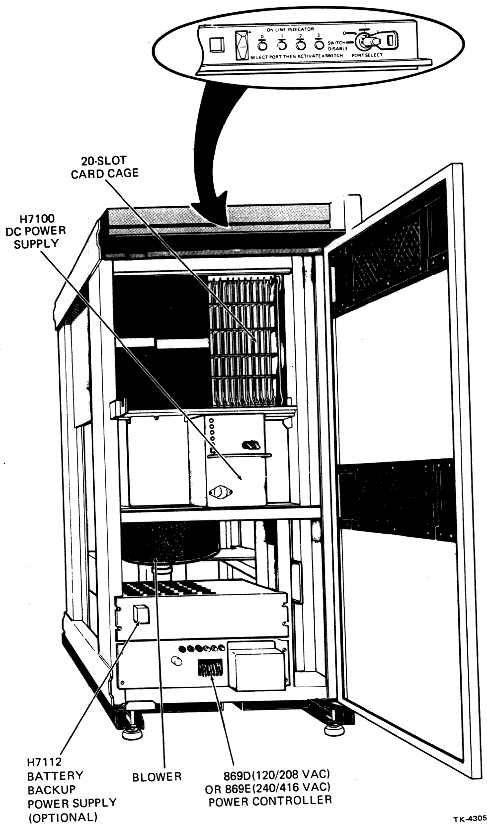
Figure 9-23 MA780 Multiport Memory Cabinet (Front View)
