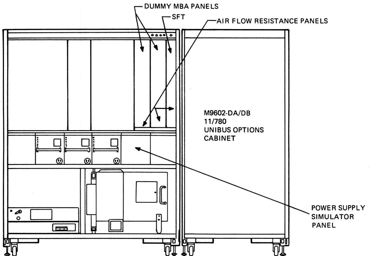
Figure 10-2 Standard VAX (SV-AXHHA) Cabinet Configuration (Front View)
