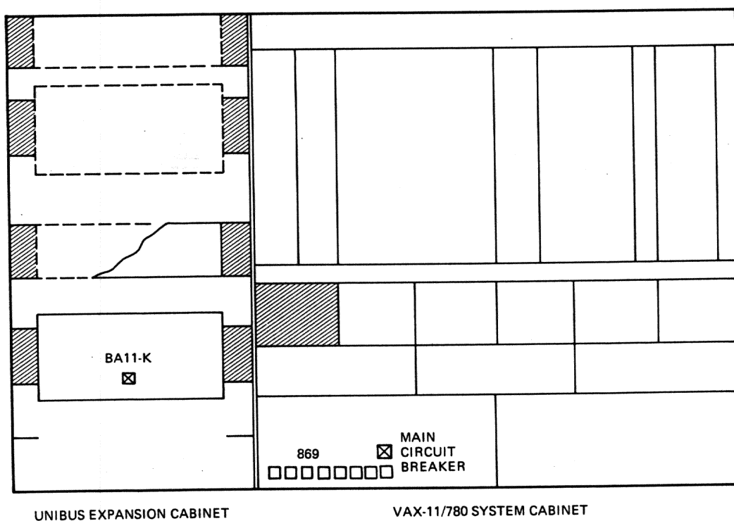
REAR VIEW
