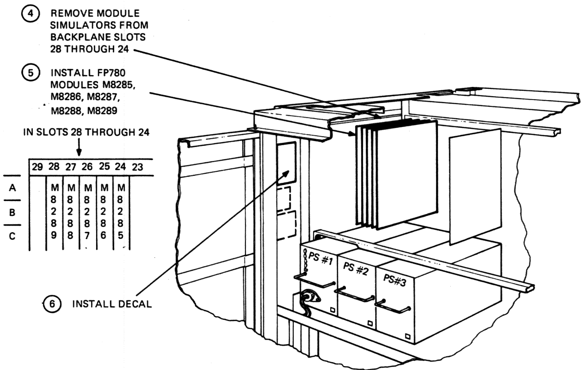
Figure 4-2 FP780 Installation (Sheet 2 of 4)
