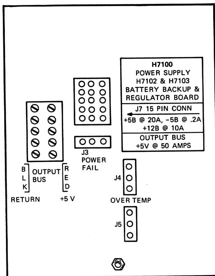
Figure 9-27 Memory Power Supply (Back View)
