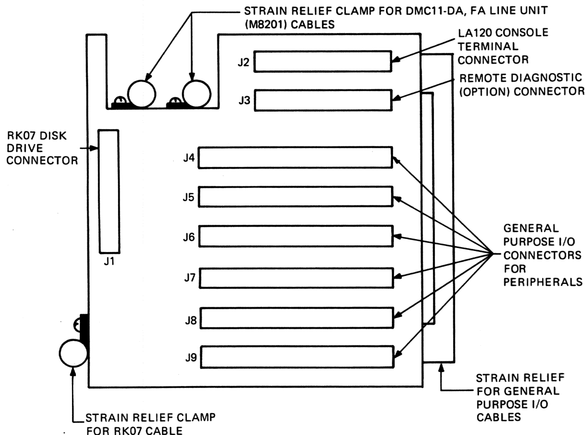
Figure 10-4 I/O Panel Assembly Connectors
