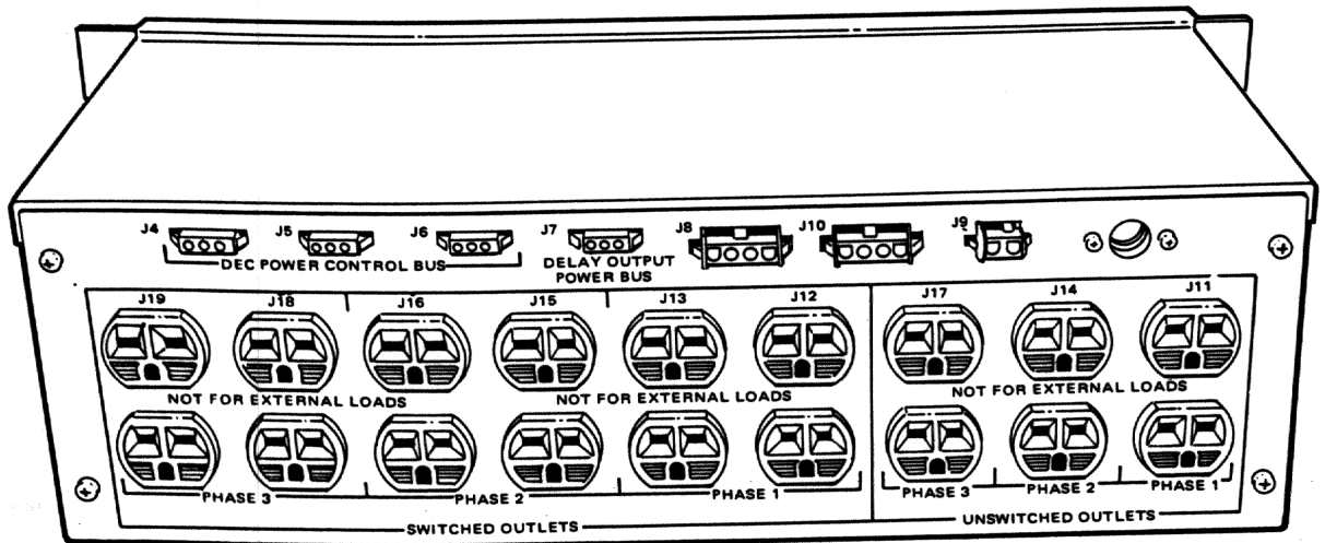
Figure 9-32 869E Power Controller (Front and Back Views)
