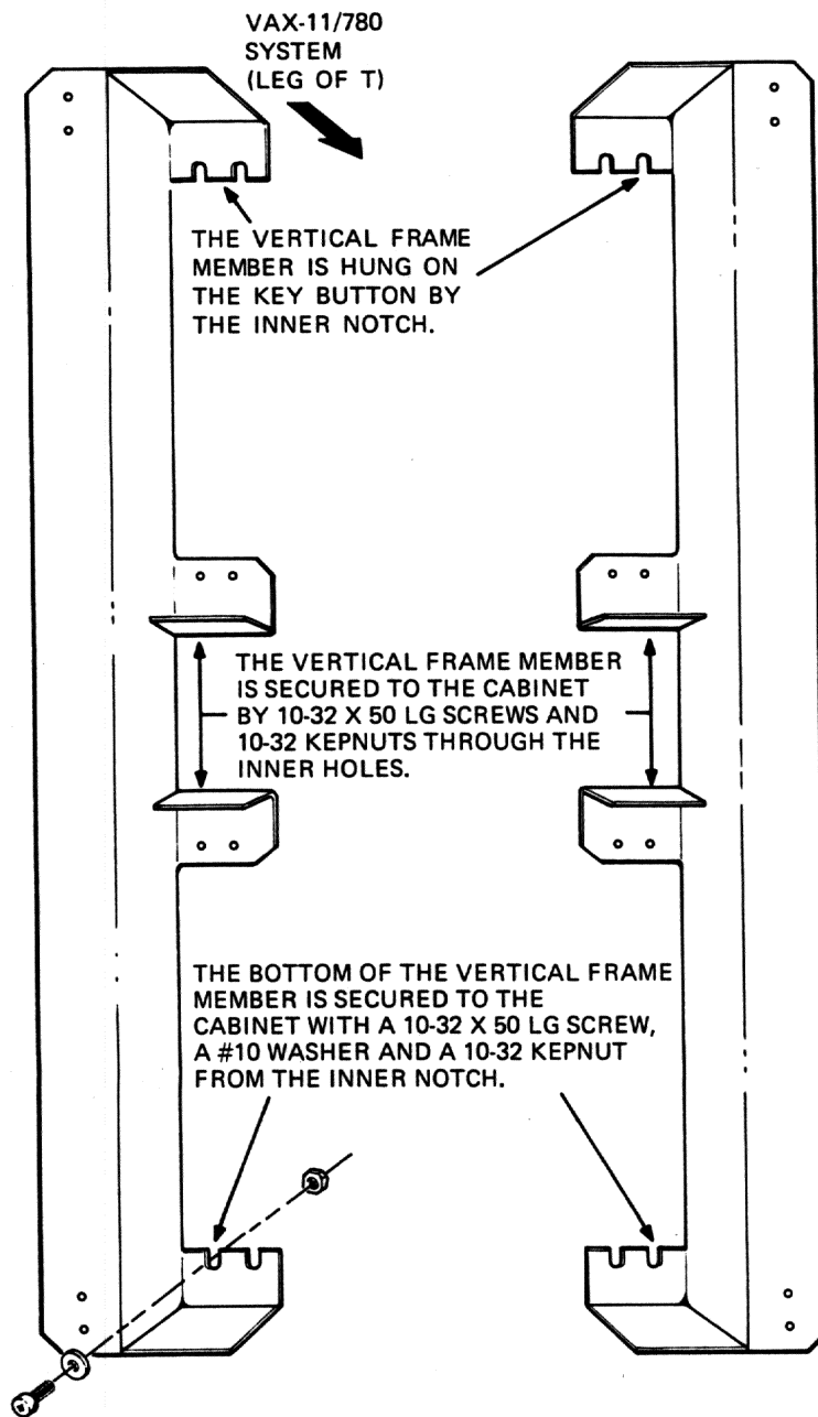
Figure 9-7 H9504-XE Vertical Frame Member Installation
