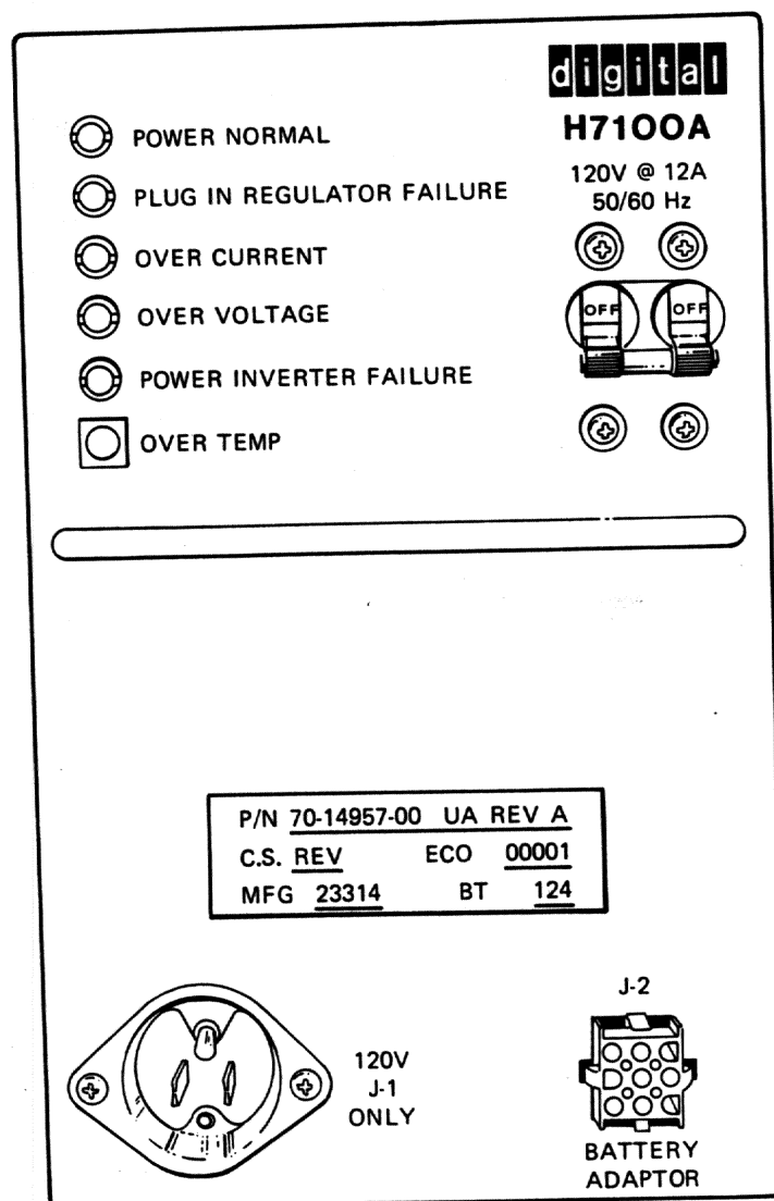
Figure 9-29 Memory Power Supply (Front View)
