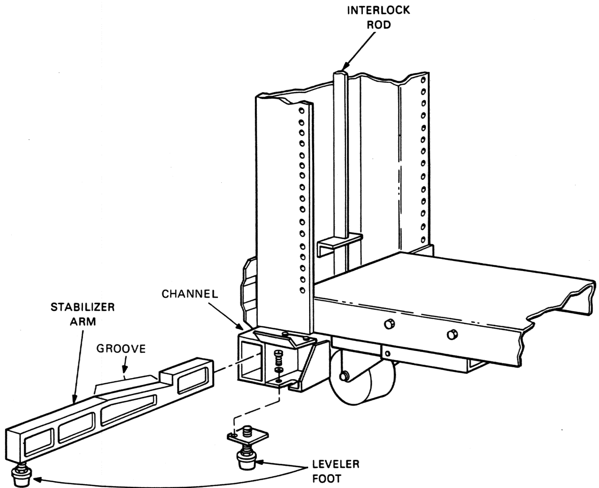
Figure 1-6 Stabilizer Arm and Leveling Pad
