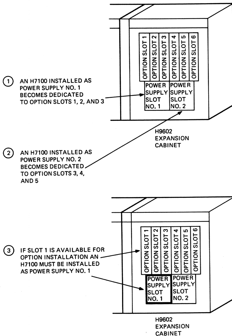
Figure 5-1 Power Supply Utilization (Sheet 1 of 2)
