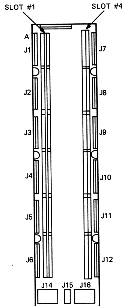
Figure 9-19 MA780C Back View
