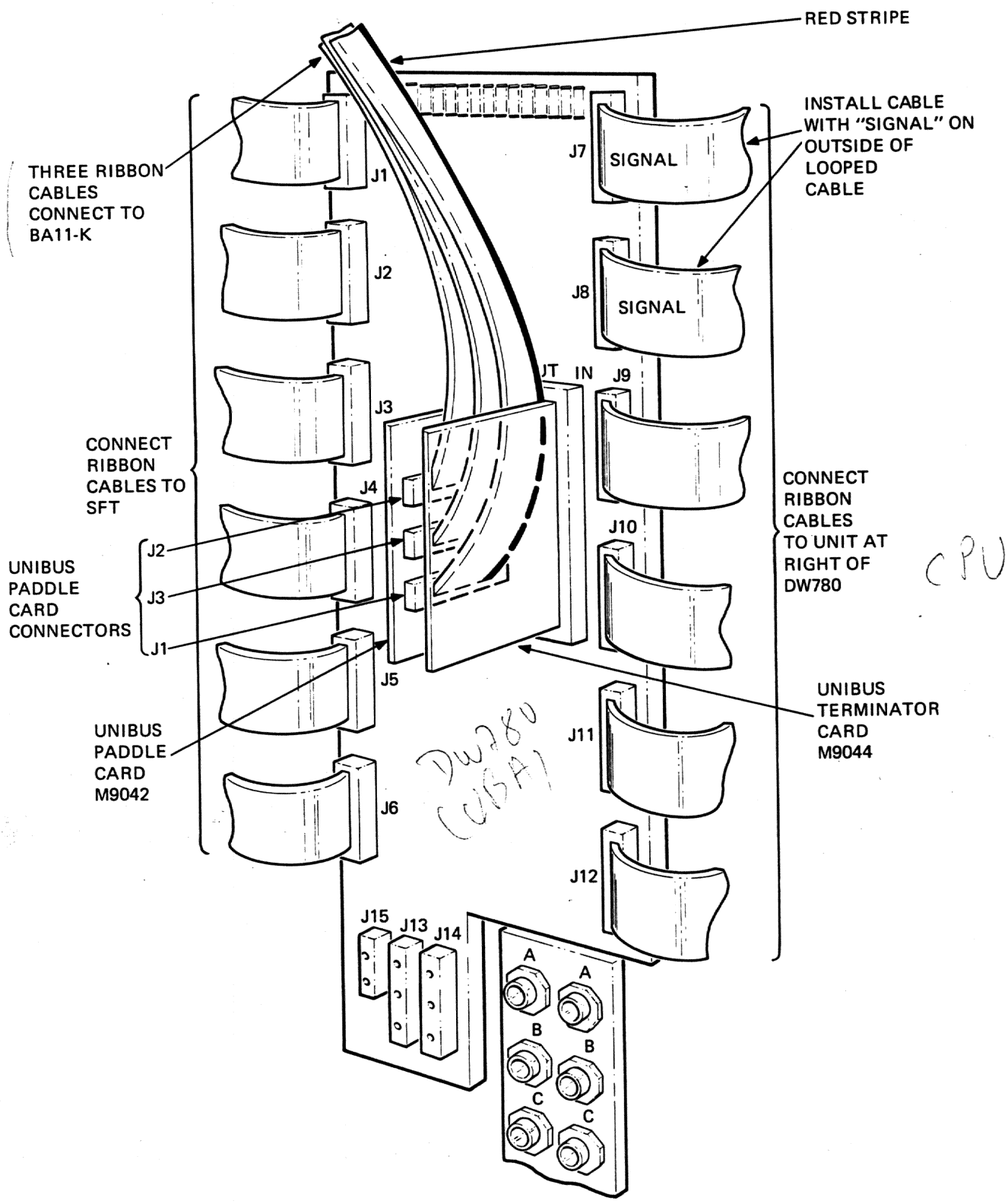
Figure 5-3 DW780 Installation Details
