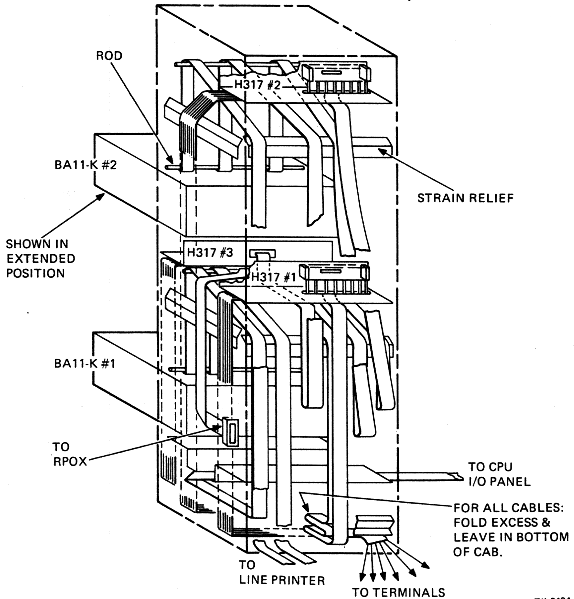
Figure 1-8 UNIBUS Expander Cabinet Cabling
