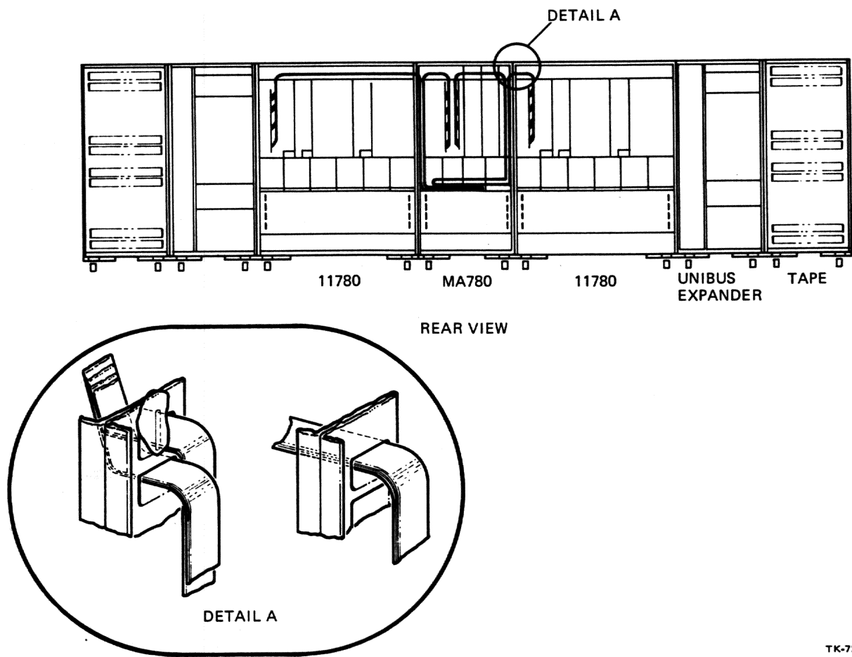
Figure 9-2 Two-System BDI Cable Routing
