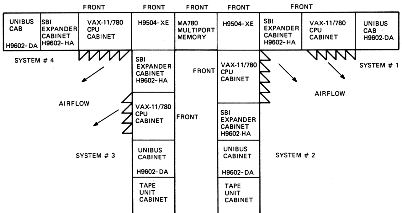
Figure 9-15 Four VAX-11/780 Systems in a “pi” Configuration
