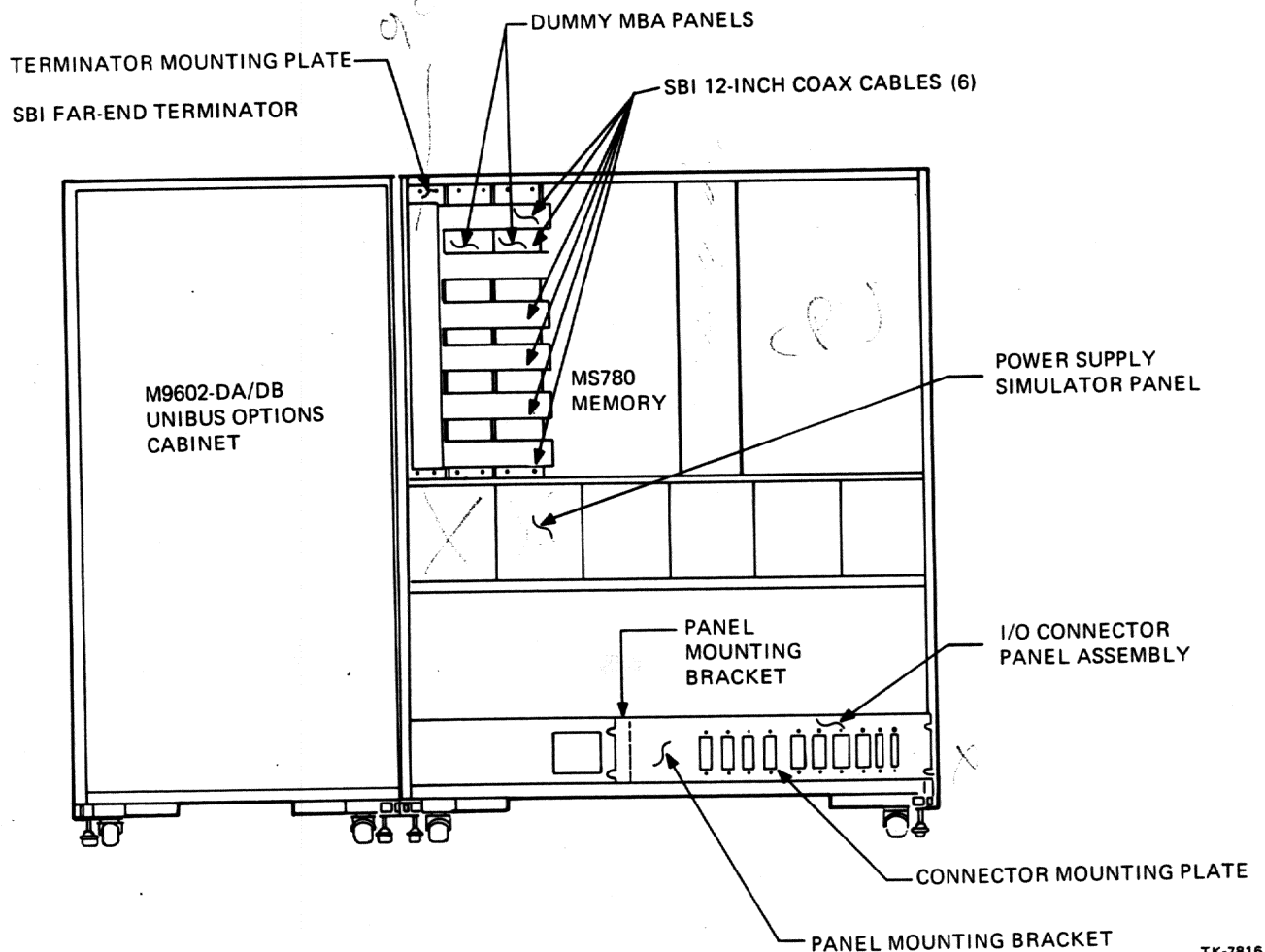
Figure 12-2 Standard VAX (SV-AXHHA) Cabinet Configuration
