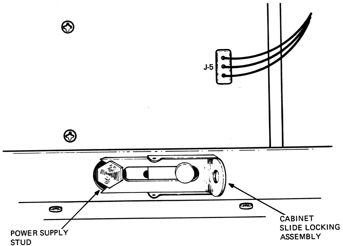
Figure 5-2 Power Supply Slidelock Details
