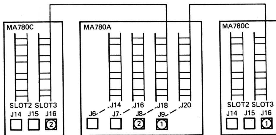
Figure 9-2 Two-System BDI Cable Routing
