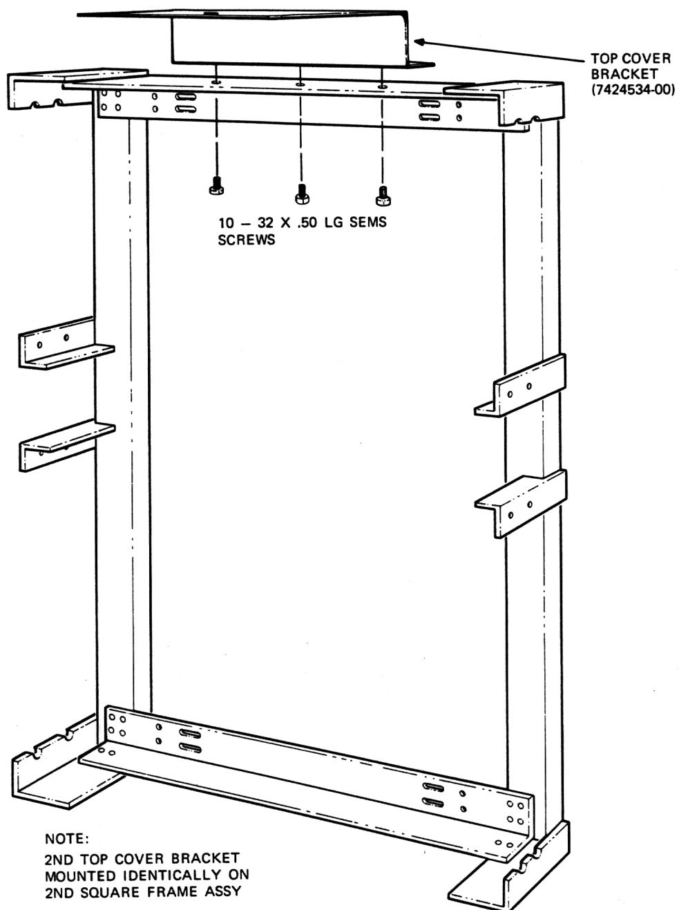
Figure 9-9 H9504-XE Top Cover Bracket Installation
