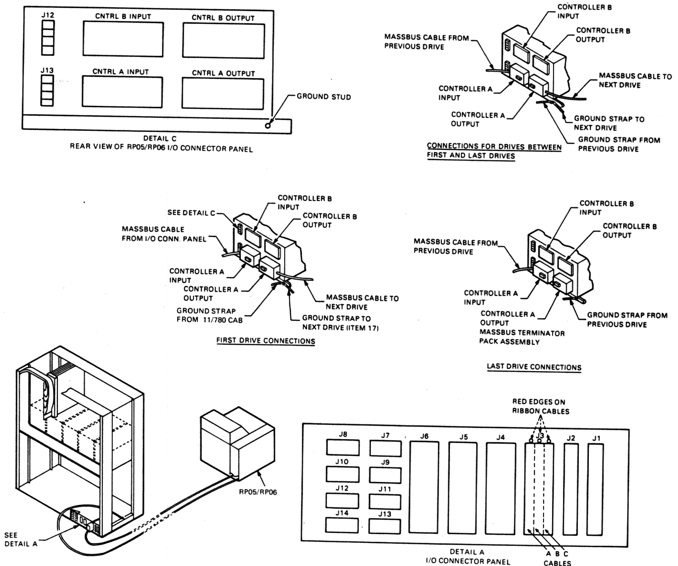
Figure 1-10 RP05/RP06 Cable Connections
