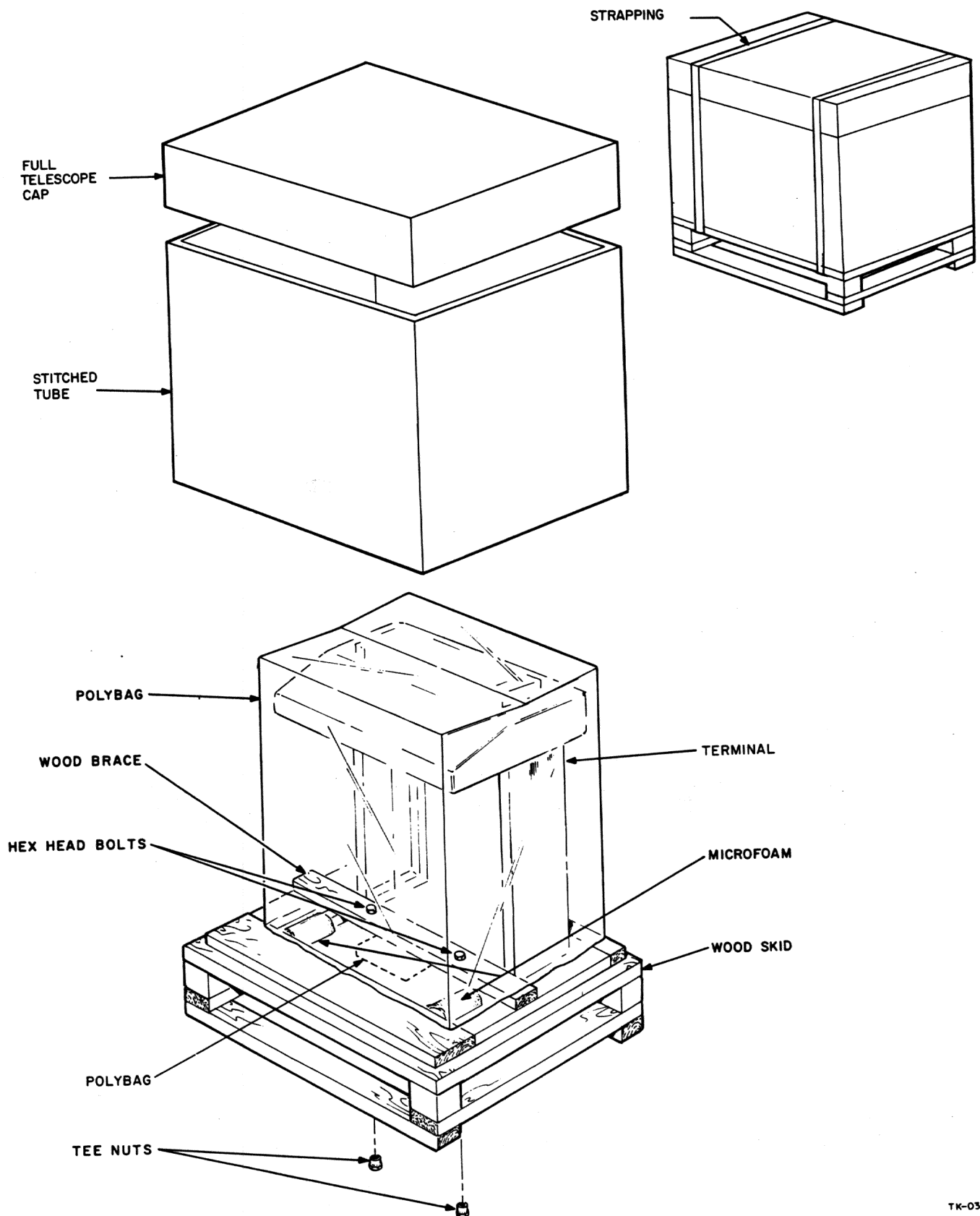
Figure 1-13 Console Packaging
