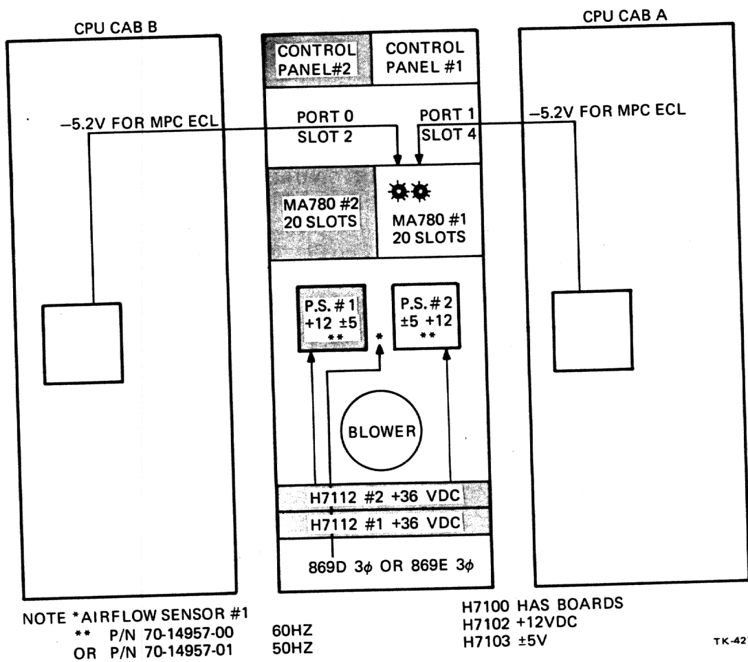
Figure 9-25 MA780A (#1) and MA780B (#2) Physical Location
