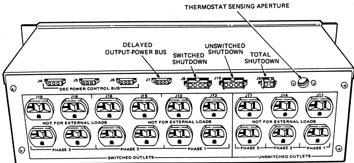
Figure 9-31 869D Power Controller (Front and Back Views)
