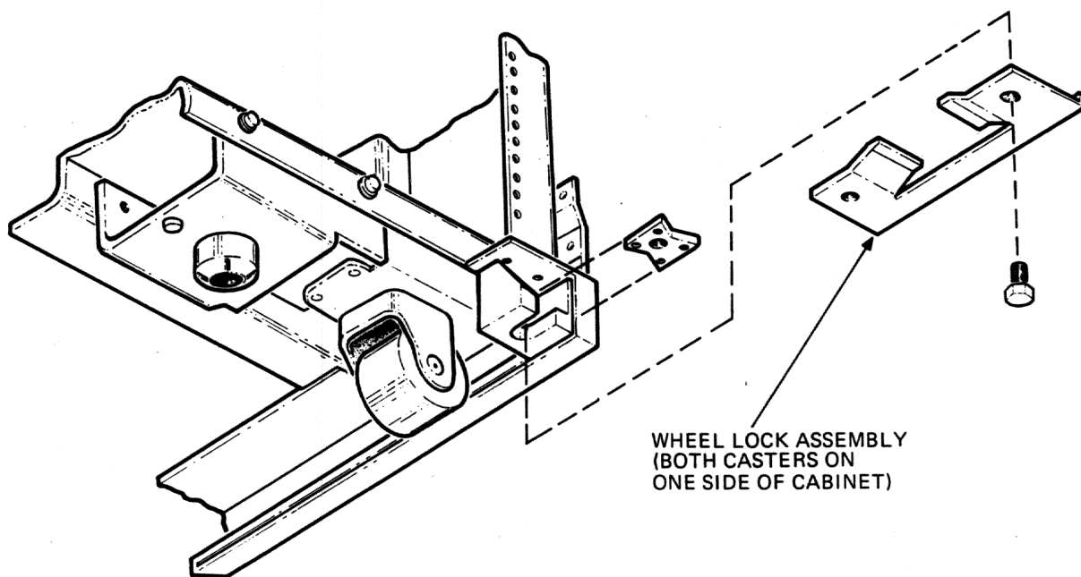
Figure 1-3 Wheel Lock Assembly
