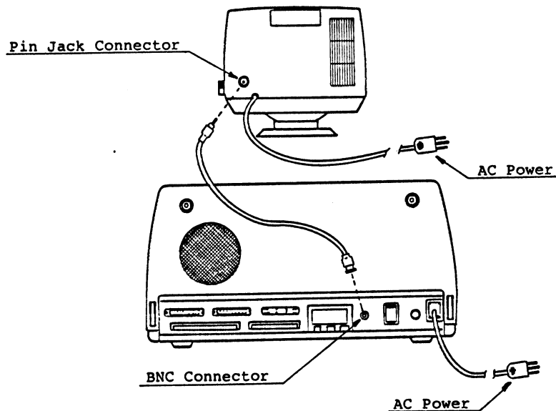
Fig. 8 : FM-9 Cable Connection
