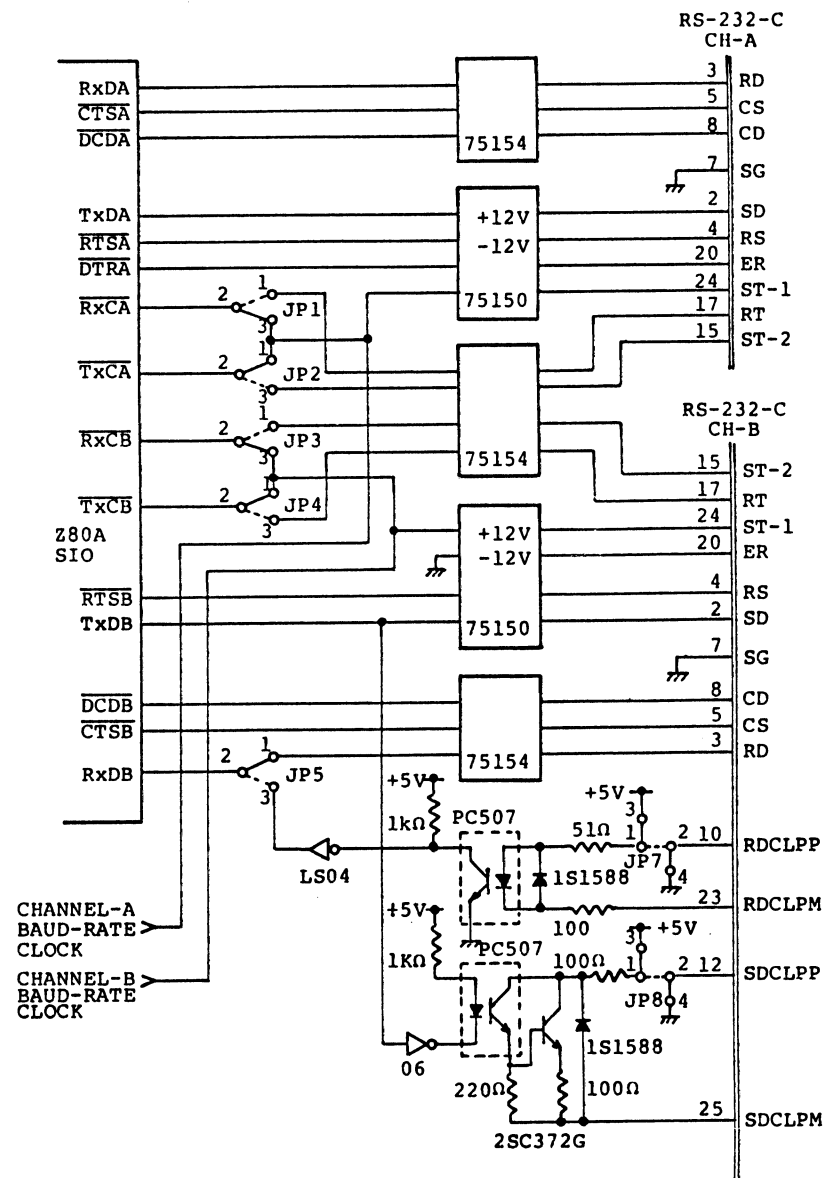
Fig. 6 : Logic of Serial I/O Ports
