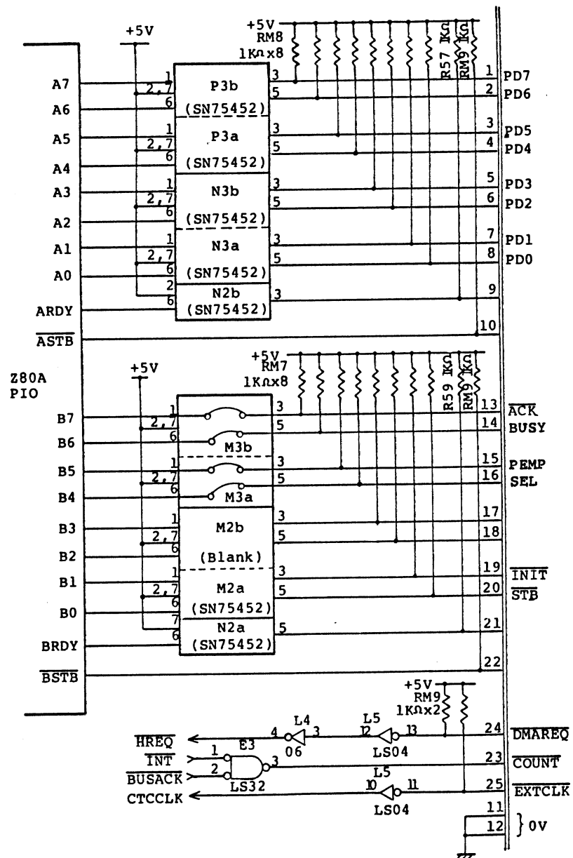
Fig. 4 : Logic of Parallel I/O Ports
