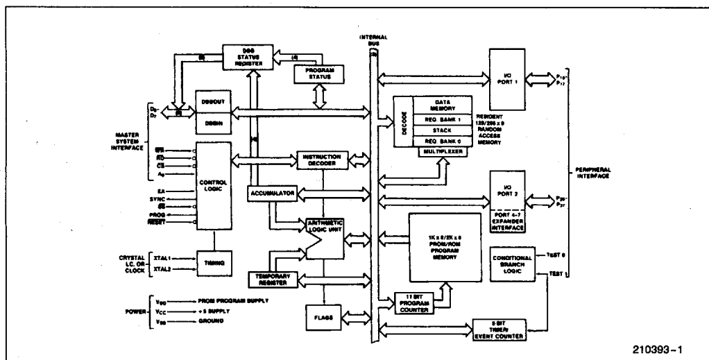
Figure 3. Block Diagram
