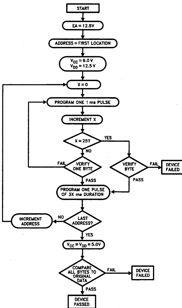
Figure 9. Programming Algorithm
