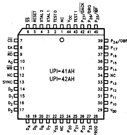
Figure 2. PLCC Pin Configuration
