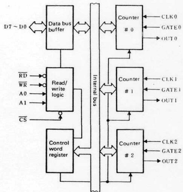
Block diagram
