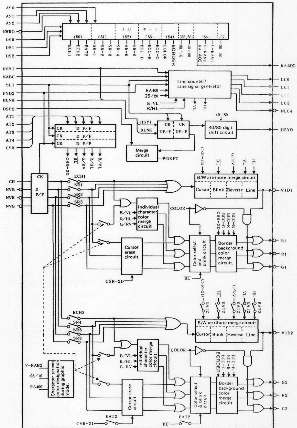
CSP-1 Block Diagram
