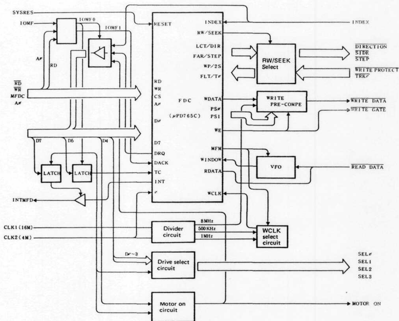
5-3. MFD interface block diagram
